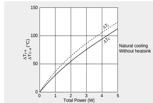
Fig. 8 Temperature rise
