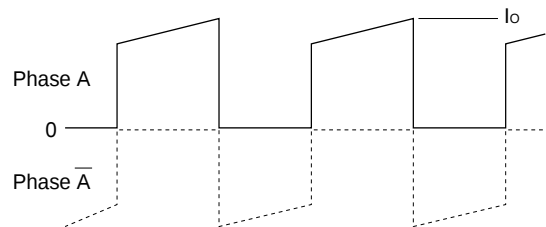
Fig. 1 Waveform of coil current (Phase A excitation ON)
