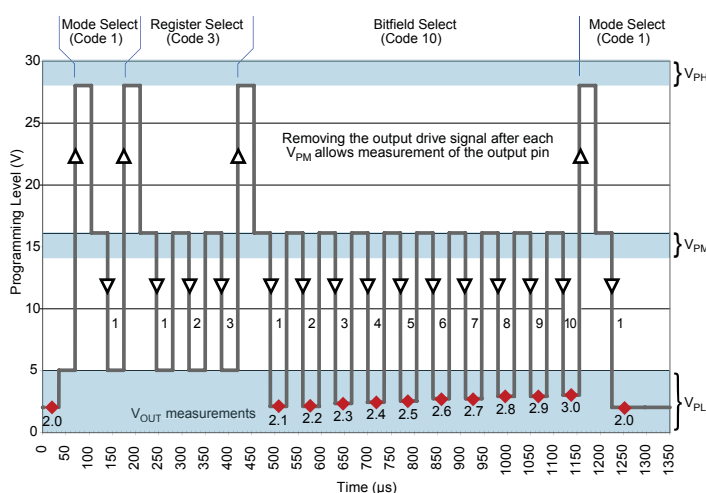
B. Try Value Mode. Code search with drive signal released after each V_{PM} , allows output to be measured after each code increment.
