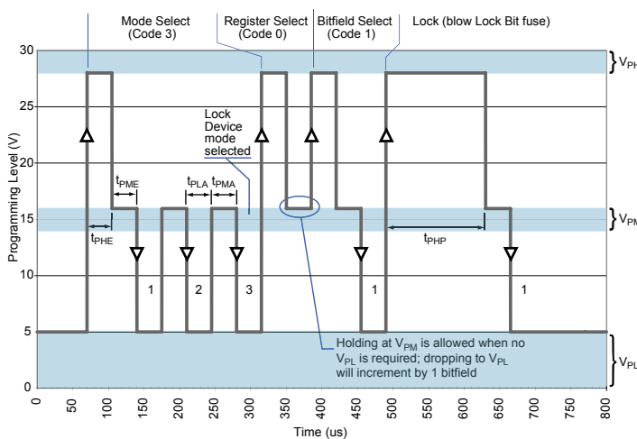
D. Lock Device Mode. Device-level Lock Bit is programmed; device programming is then permanently disabled.
