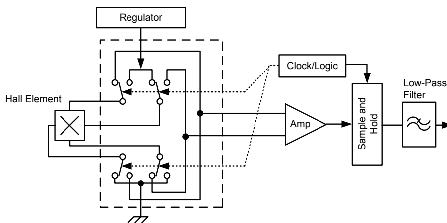
Concept of Chopper Stabilization Technique
