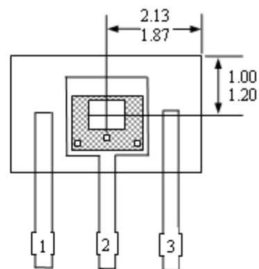
Sensor Location
