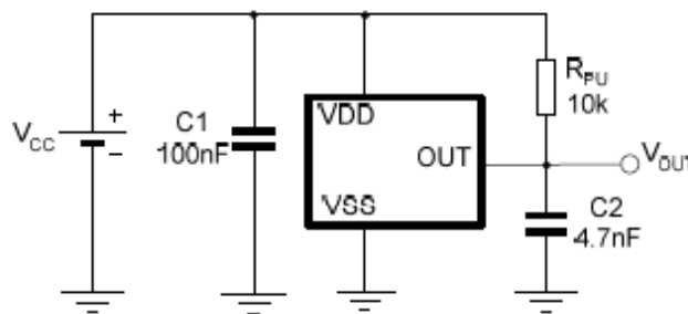
Typical Three-Wire Application Circuit
