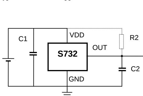
Typical Three-Wire Application Circuit
