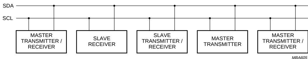
Fig 10. System configuration.
