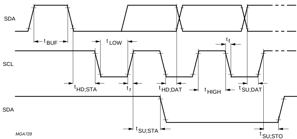
Fig 16. I²C-bus timing waveforms.
