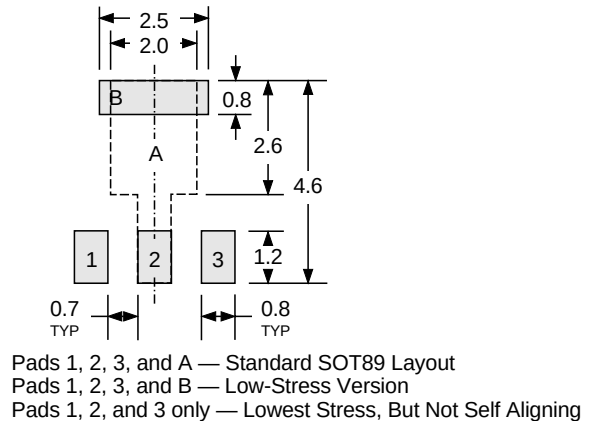
Dwg. MA-012-3 mm
