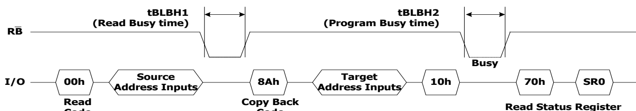
Figure 15. Copy Back Operation
