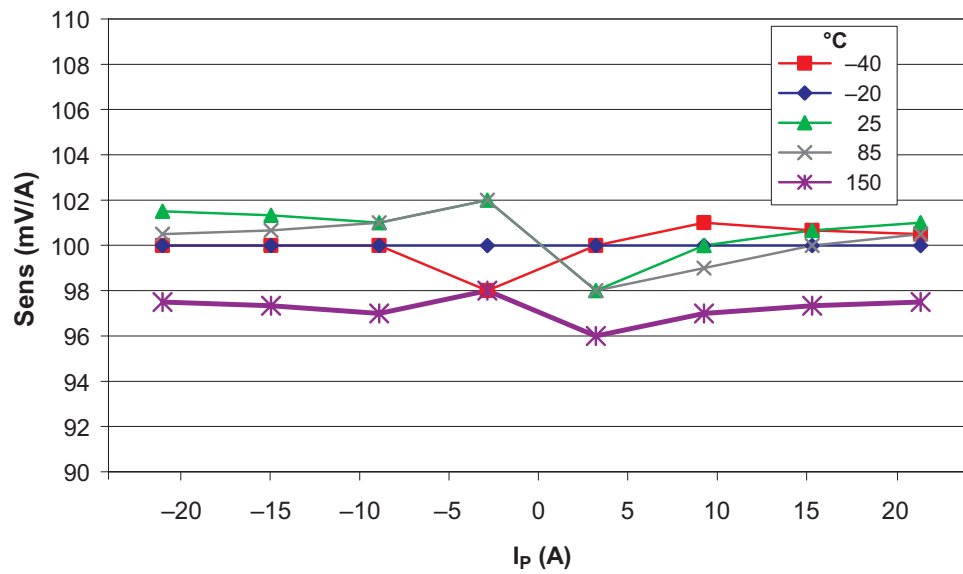
Sensitivity versus Primary Current
