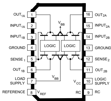
A3968SLB (SOIC)
