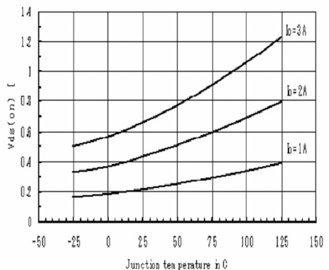
Normalized FET on resistance
