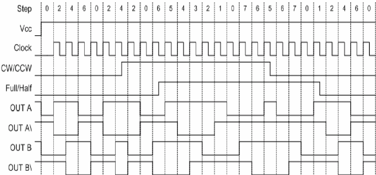
Timing chart
