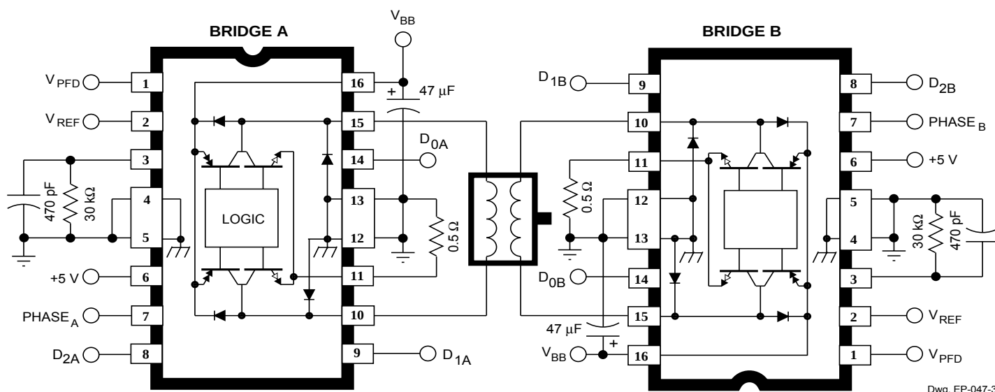
Figure 4 — Typical Application
