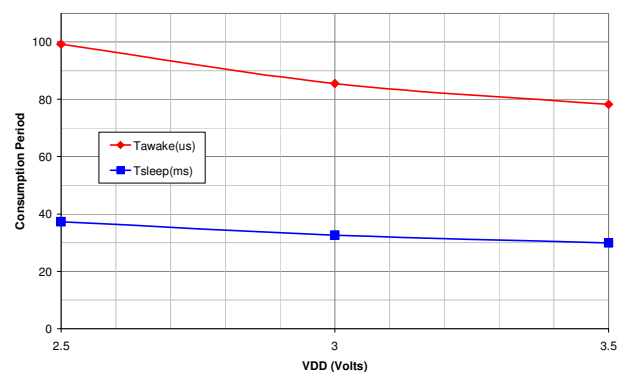
11.6 Consumption Period vs. V_{DD}
