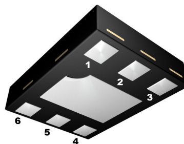
LD Package
