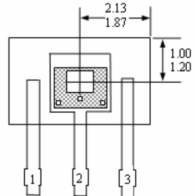
Sensor Location
