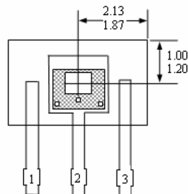
Sensor Location
